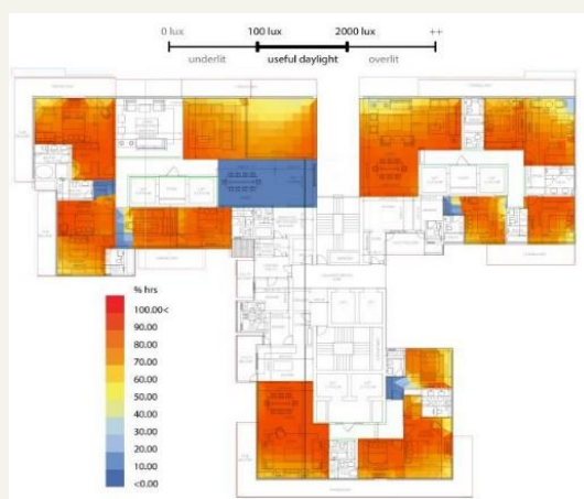
Figure 4.1 UDI Analysis with a Daylighting Analysis Software
